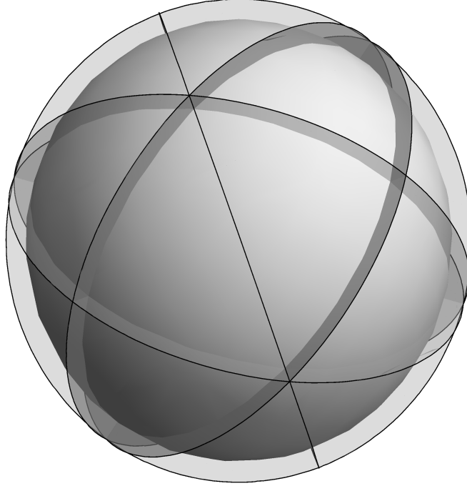
FIGURE 8. \mathcal{N} for the collinear four-body problem. The collision planes divide the sphere into triangles representing the possible orderings of the bodies.
