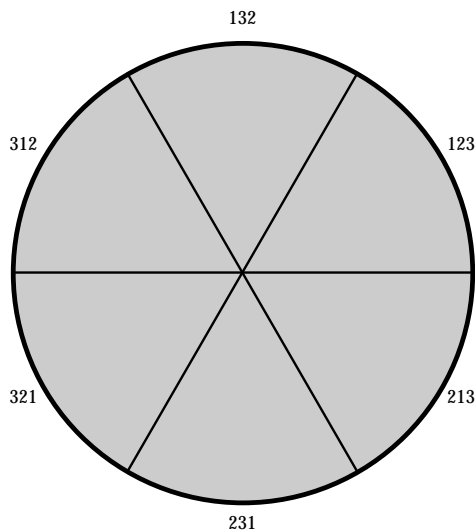
FIGURE 7. \mathcal{N} for the collinear three-body problem is the boundary circle of the shaded disk which represents the set I \leq 1 in the plane of centered configurations. \Delta intersects this plane in three lines which divide the circle into six arcs, one for each ordering of the bodies along the line.
