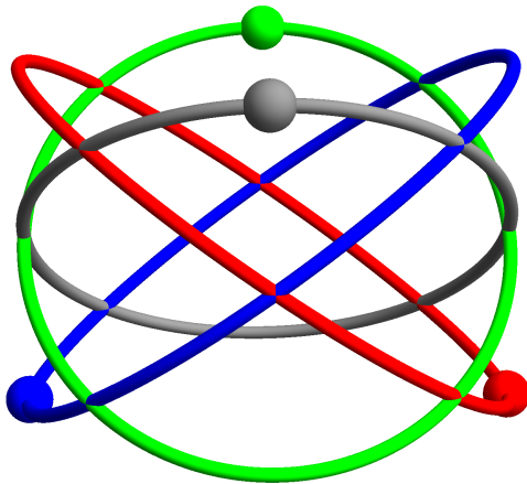
FIGURE 4. Three-dimensional projection of a rigid motion of a central configuration in \mathbb{R}^4 . Four equal masses are at the vertices of a regular tetrahedron. Each body moves on a circle in \mathbb{R}^4 but the circles are in different planes. In the projection, the circles become ellipses.
