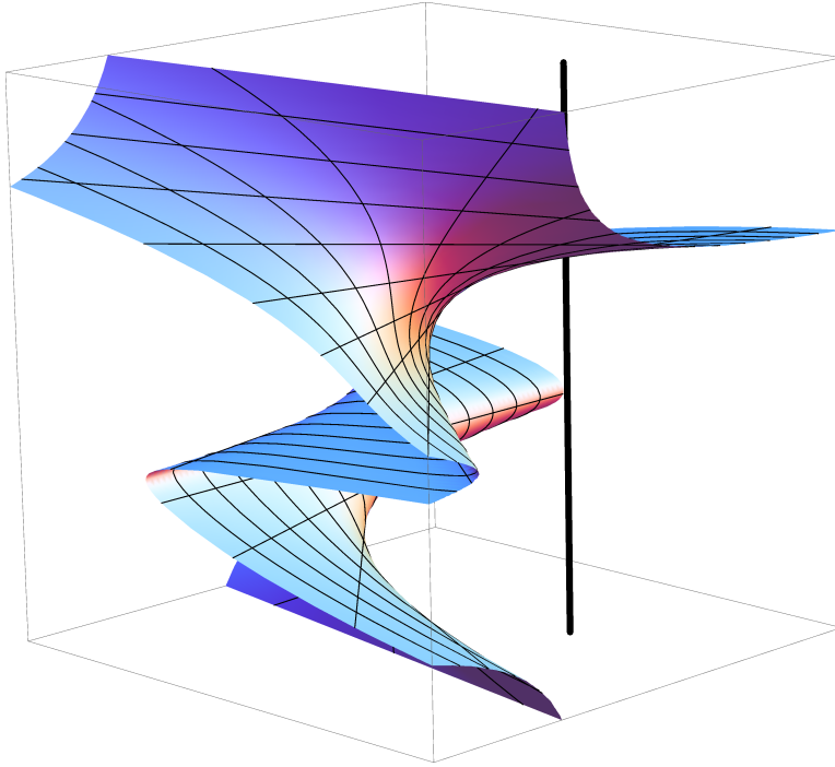
FIGURE 6. Surface defined by Euler's quintic equations in the product space of masses and configurations. Two mass parameters (horizontal) and one configuration variable r (vertical). Fixing the masses means looking for intersections of the surface with a vertical fiber, here a line segment. For positive masses, the segment cuts the surface just once.
