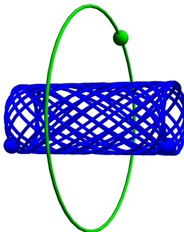
FIGURE 5. Three-dimensional projection of a rigid motion of a balanced configuration in \mathbb{R}^4 . An isosceles triangle with edges 1, \frac{\sqrt{3}}{2}, \frac{\sqrt{3}}{2} and masses 1, 1, \frac{\sqrt{5}-1}{2} is rotating with different frequencies in two orthogonal planes in \mathbb{R}^4 . The mass on the symmetry axis is in one of the planes and moves on a circle while the other two masses move on a torus.
