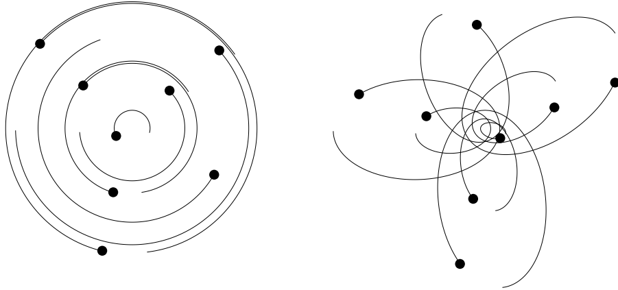
FIGURE 3. Planar homographic motions based on a central configuration of eight equal masses from figure 1. On the left is a relative equilibrium solution while the solution on the right features elliptical orbits of eccentricity 0.8
