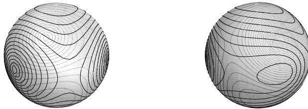
FIGURE 9. \mathcal{M} for the planar three-body problem is the shape sphere. The Newtonian potential determines a Morse function with five critical points, shown here for the case of equal masses (left) and masses 1, 2, 10 (right).
